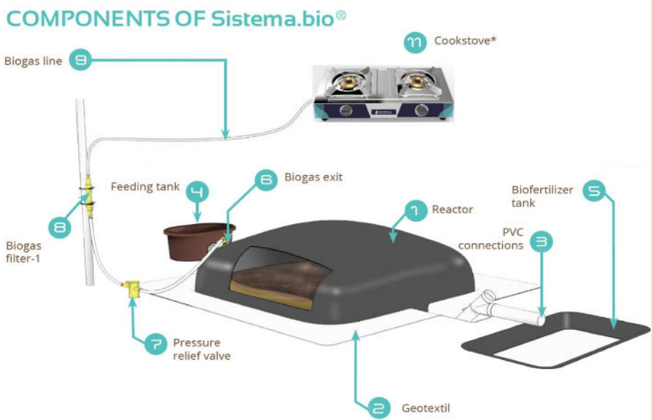
Figure 1: Sistema.bio's biodigester displaying its components and main features
